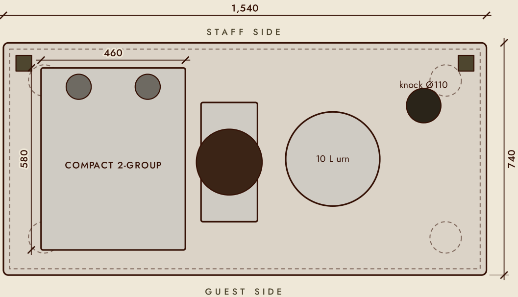
PLAN · SET-UP B · COFFEE AND TEA
